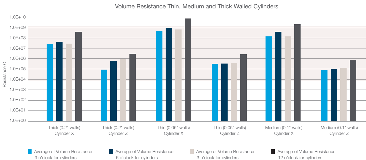
Figure 2. Volume resistance of hollow cylinders with respect to wall thickness, build orientation, and location on the cylinder.
